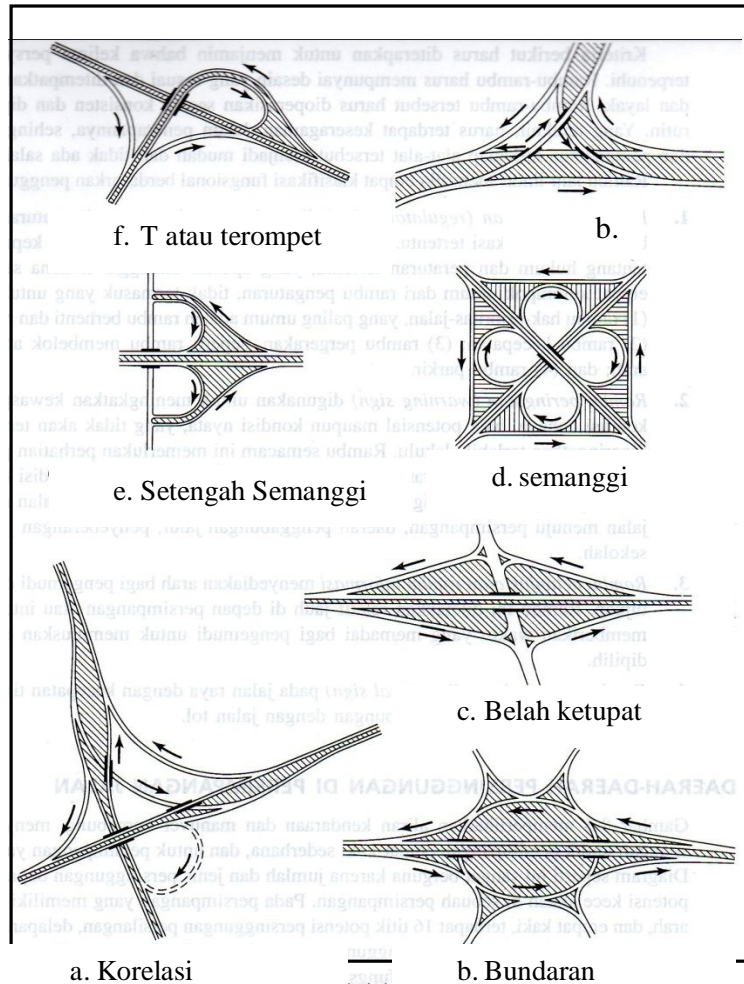
Figure 1. Types of Interchange Source: Khisty, 2002
